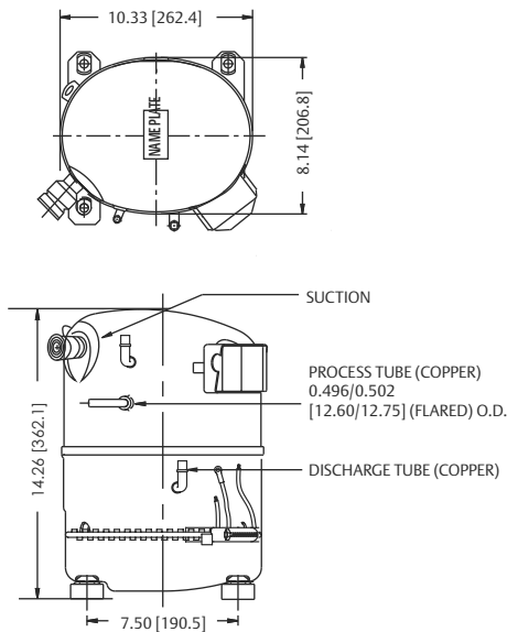
KCM515LAL/519CAL/522CAL with Spud
