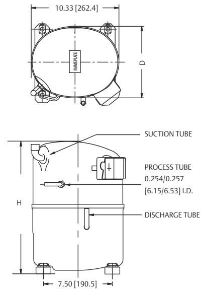
KCM515LAL/522CAL with Suction Tube
