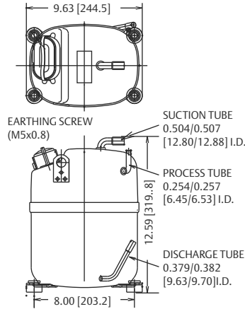
KCJ***CAL with Suction Tube
