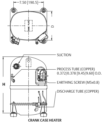
KCM475 LAL/511CAL/514CAL with Spud
