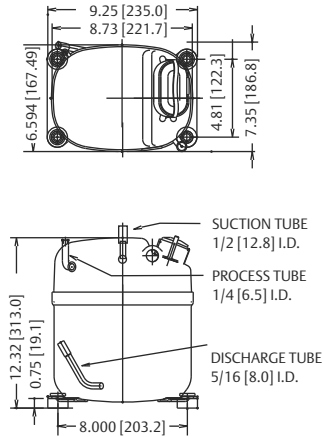
KCJ***CAL with Suction Spud
