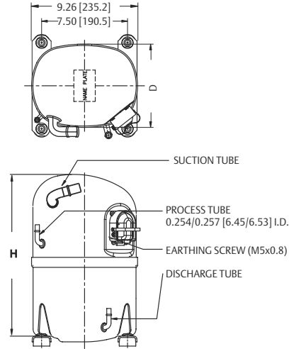
KCM475 LAL/511CAL/514CAL with Suction Tube
