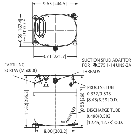
KCJ450LAL with Suction Spud
