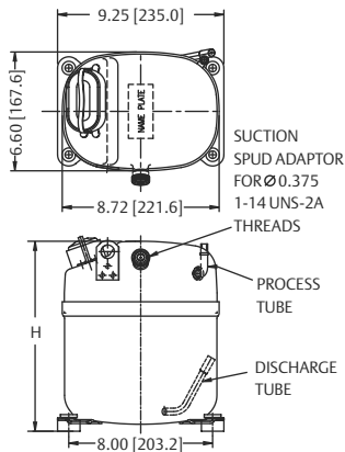
KCJ***CAL with Suction Spud
